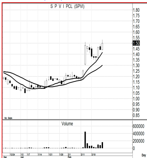
Price Chart...(SPVI)
